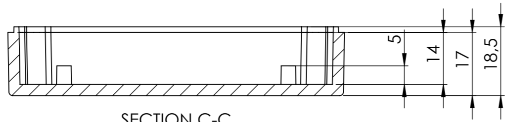
SECTION C-C
