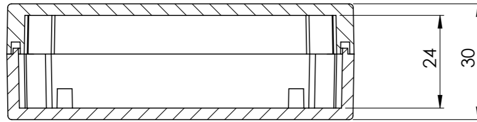
SECTION B-B
